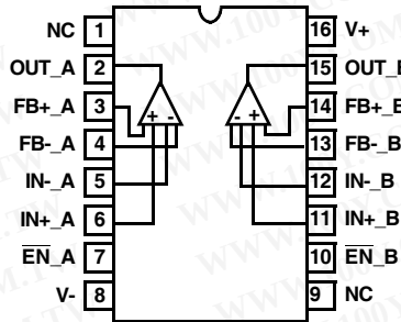
ISL28270, ISL28273 (16 LD QSOP) TOP VIEW
